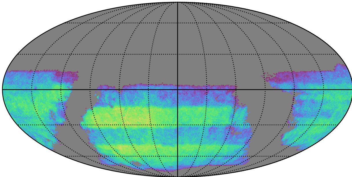
baseline_v3.4_10yrs i band non-DD year 3: ExgalM5WithCuts
