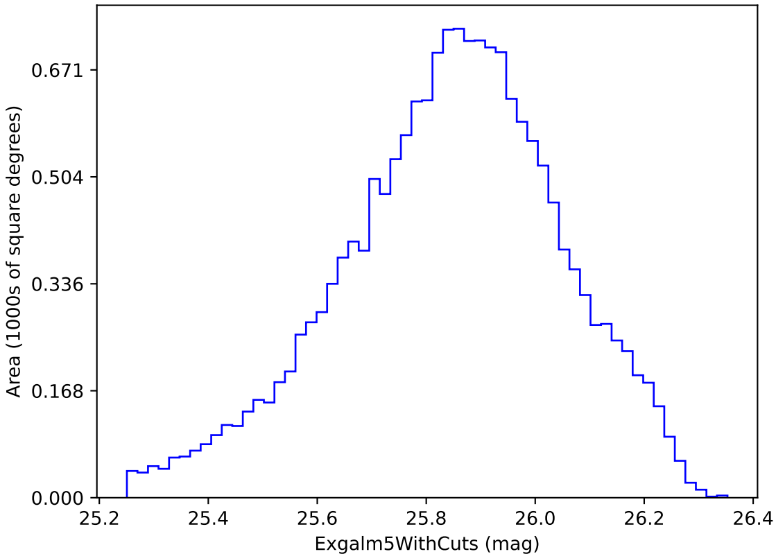
baseline_v3.4_10yrs i band non-DD year 3: ExgalM5WithCuts
