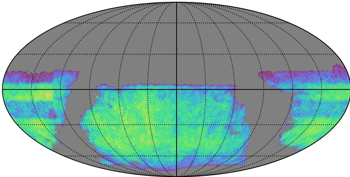
baseline_v3.4_10yrs i band non-DD year 2: ExgalM5WithCuts
