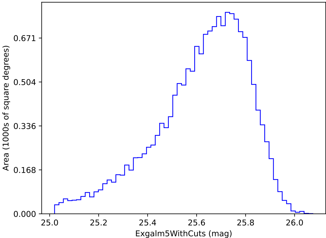
baseline_v3.4_10yrs i band non-DD year 2: ExgalM5WithCuts
