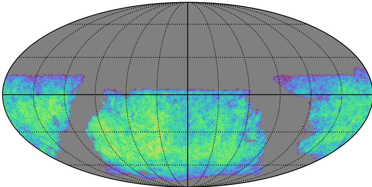
baseline_v3.4_10yrs i band non-DD year 1: ExgalM5WithCuts
