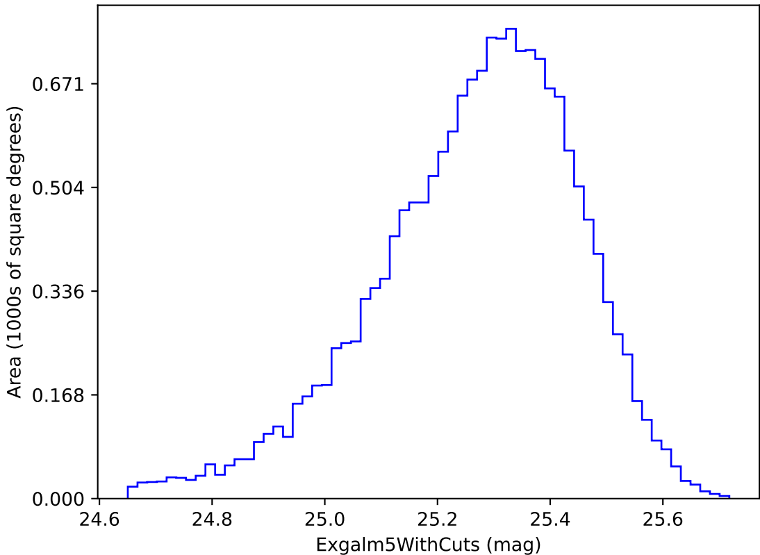
baseline_v3.4_10yrs i band non-DD year 1: ExgalM5WithCuts
