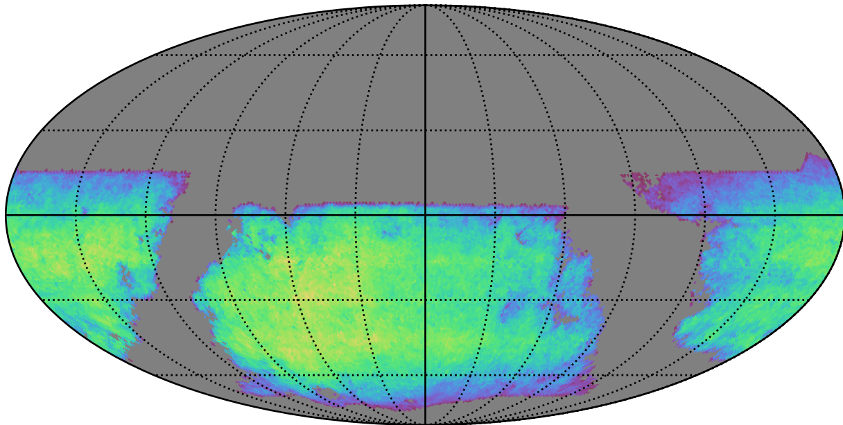
baseline_v3.4_10yrs i band non-DD year 10: ExgalM5WithCuts
