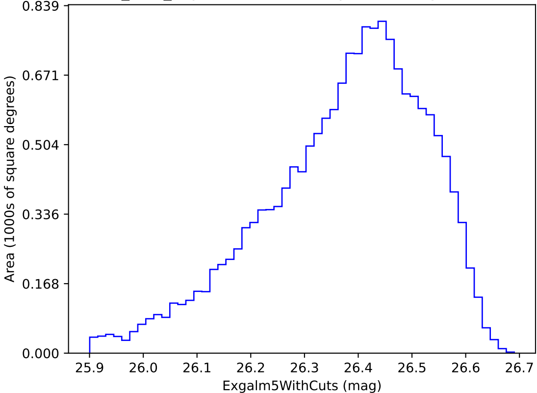
baseline_v3.4_10yrs i band non-DD year 10: ExgalM5WithCuts
