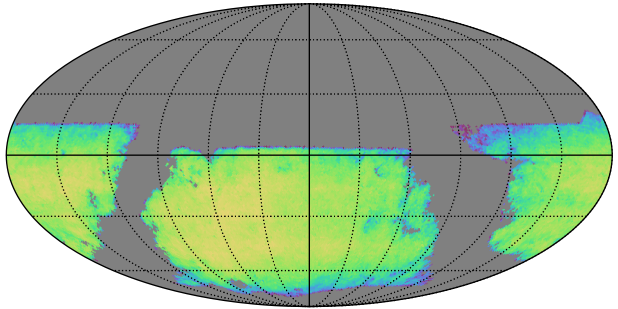
baseline_v3.4_10yrs i band galaxies non-DD: DepthLimitedNumGalaxiesMetric
