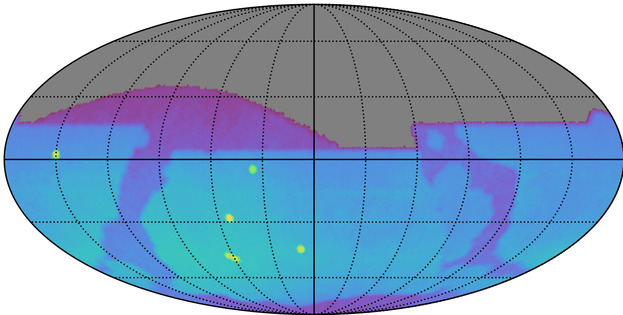
baseline_v3.4_10yrs : Brown Dwarf, L7
