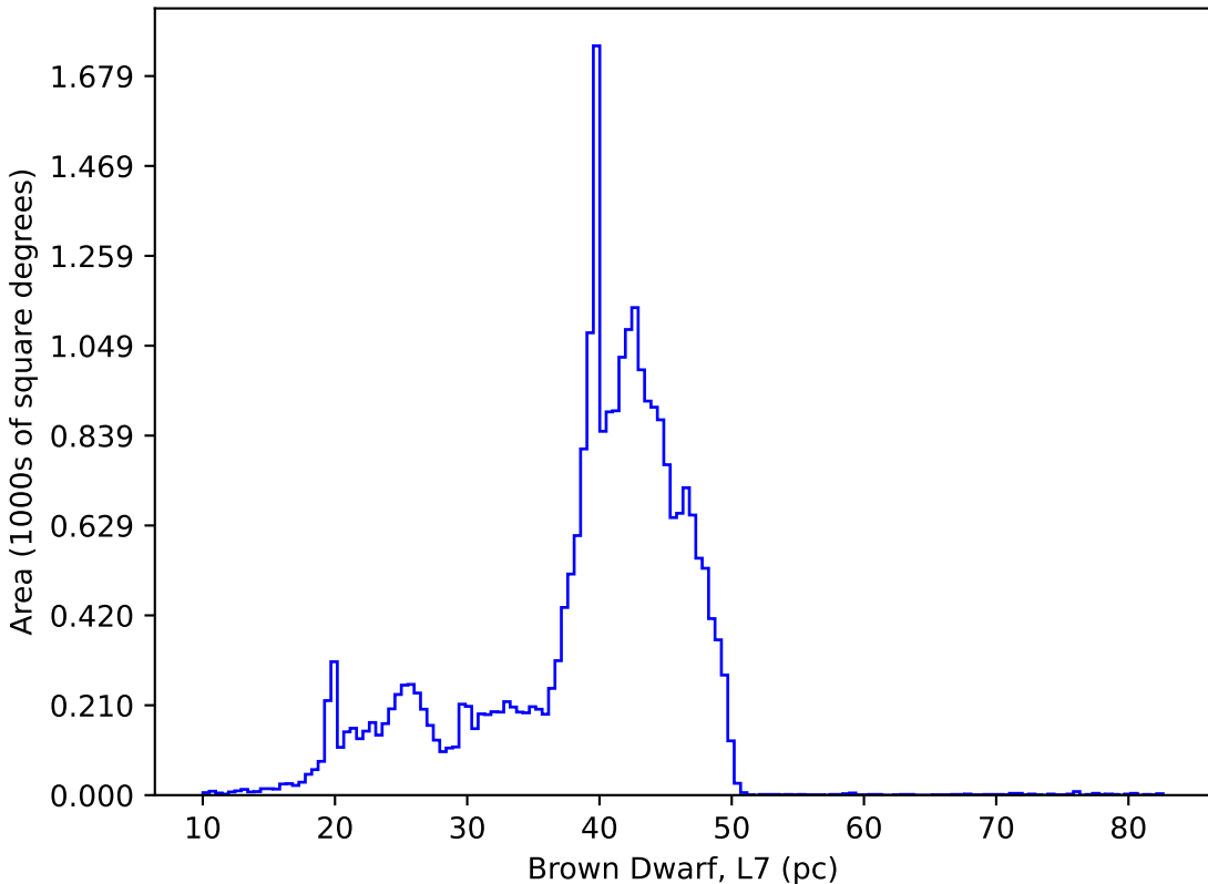
baseline_v3.4_10yrs : Brown Dwarf, L7
