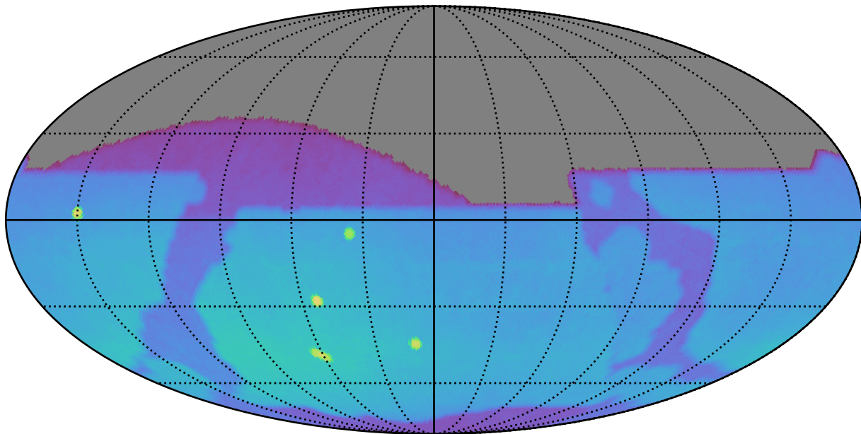
baseline_v3.4_10yrs : Brown Dwarf, L4
