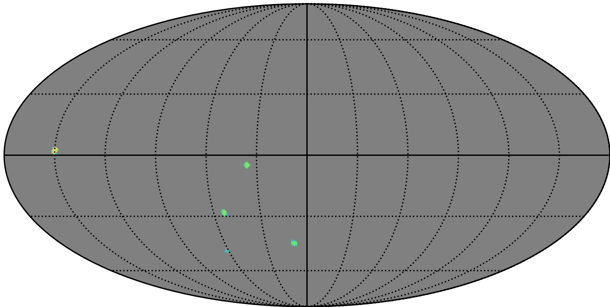
baseline_v3.4_10yrs z band: AGN_TimeLag_5_days
