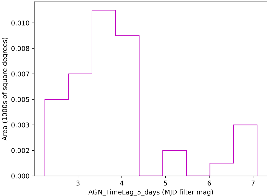
baseline_v3.4_10yrs z band: AGN_TimeLag_5_days
