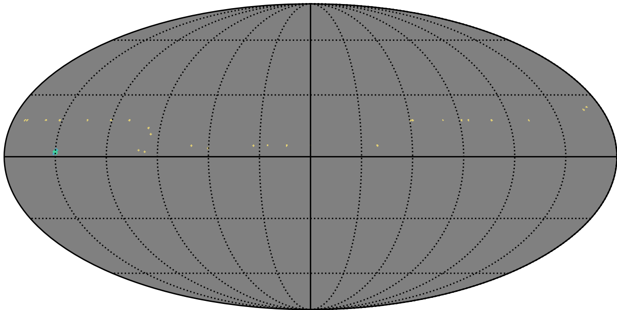
baseline_v3.4_10yrs y band: AGN_TimeLag_5_days
