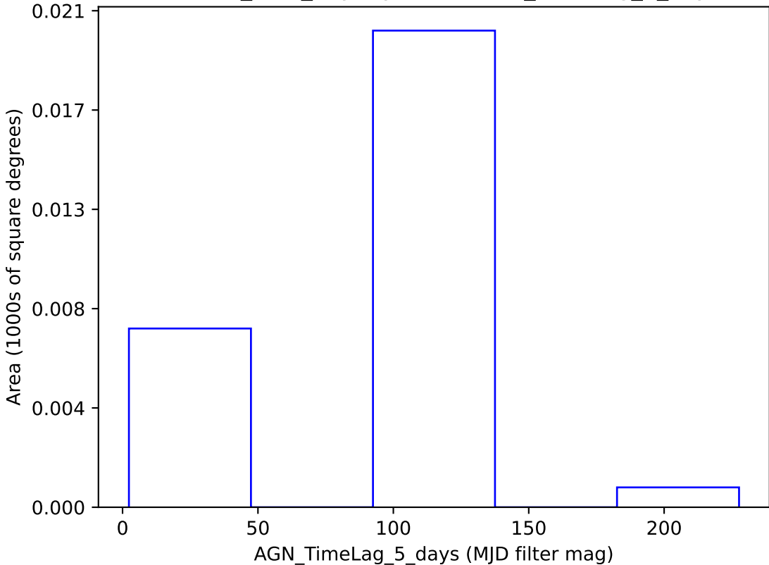
baseline_v3.4_10yrs y band: AGN_TimeLag_5_days
