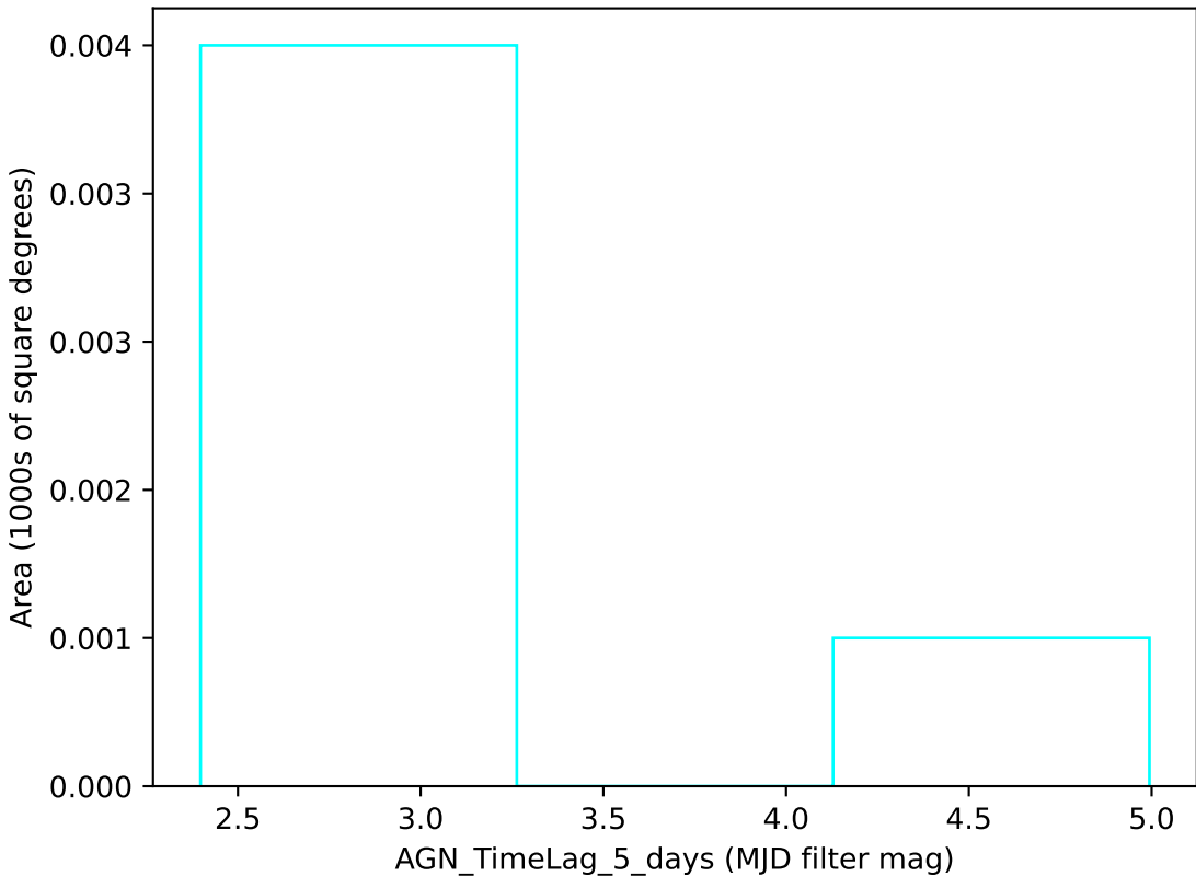
baseline_v3.4_10yrs u band: AGN_TimeLag_5_days
