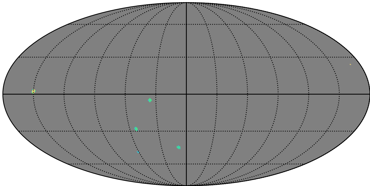
baseline_v3.4_10yrs r band: AGN_TimeLag_5_days
