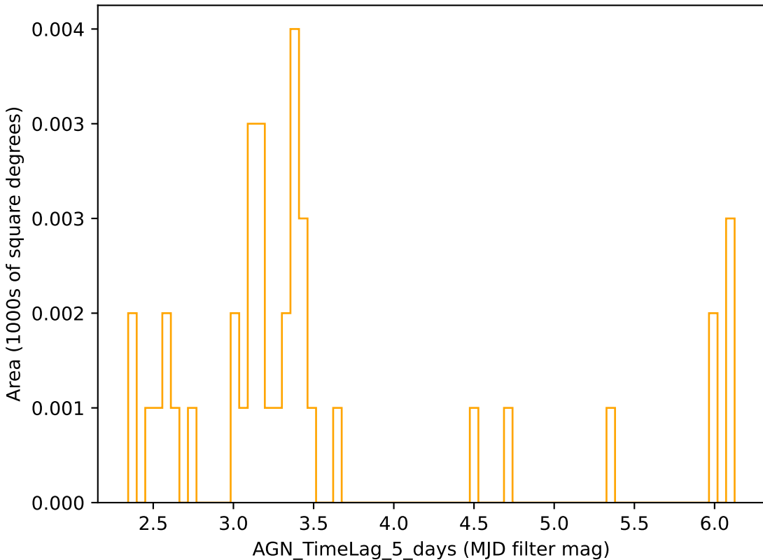
baseline_v3.4_10yrs r band: AGN_TimeLag_5_days
