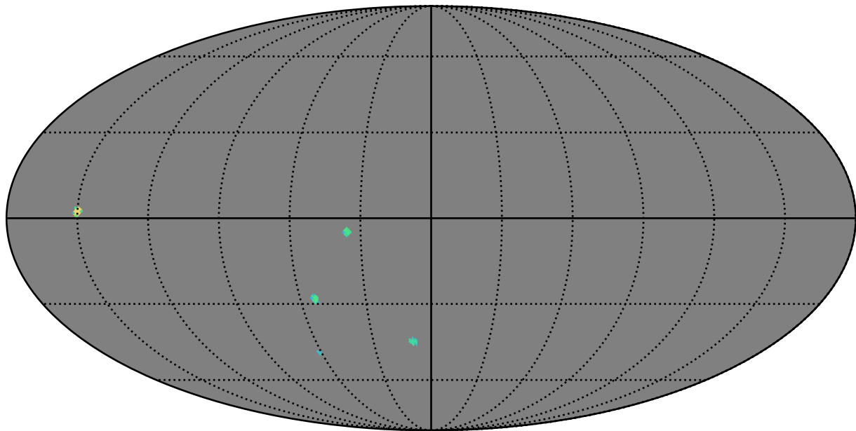
baseline_v3.4_10yrs i band: AGN_TimeLag_5_days
