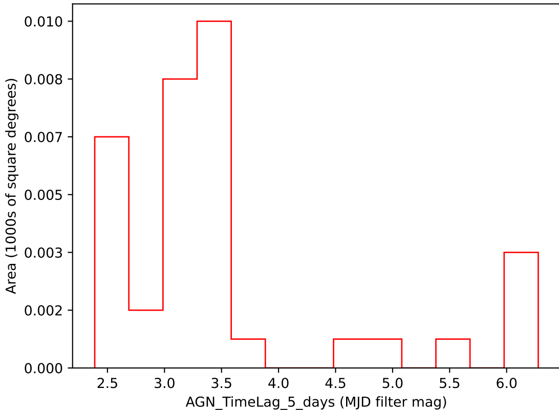
baseline_v3.4_10yrs i band: AGN_TimeLag_5_days
