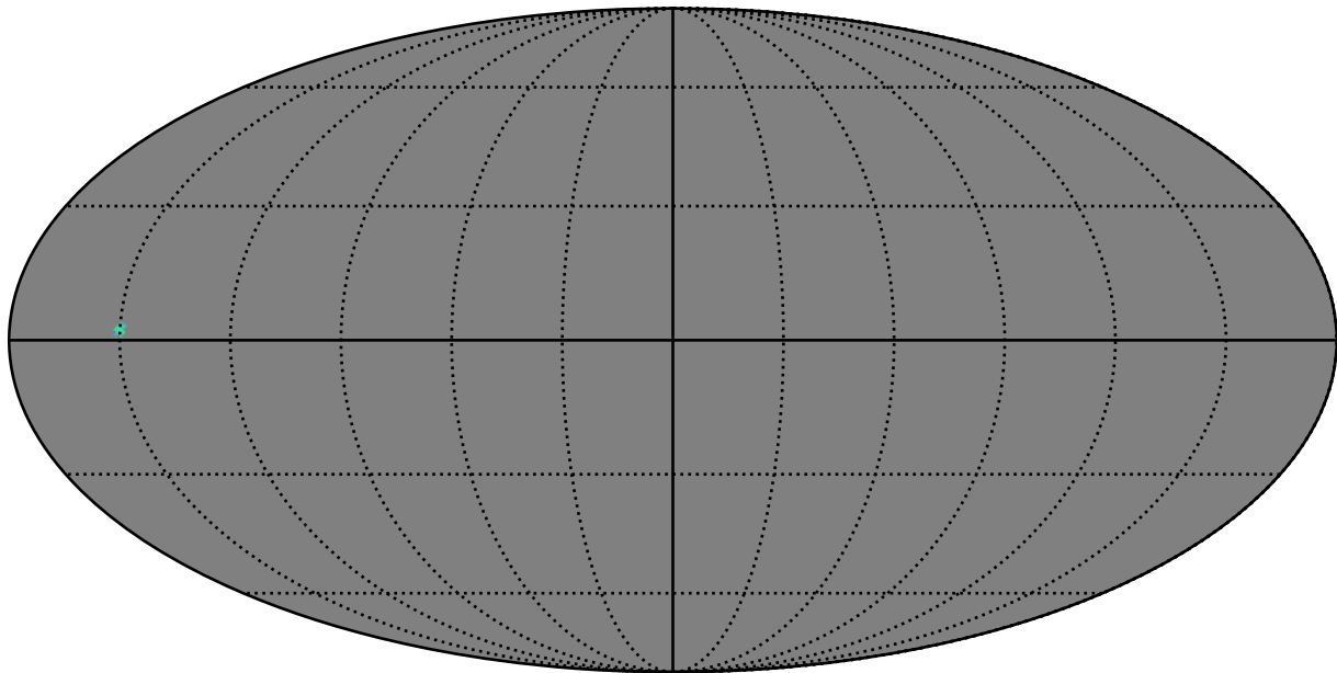
baseline_v3.4_10yrs g band: AGN_TimeLag_5_days
