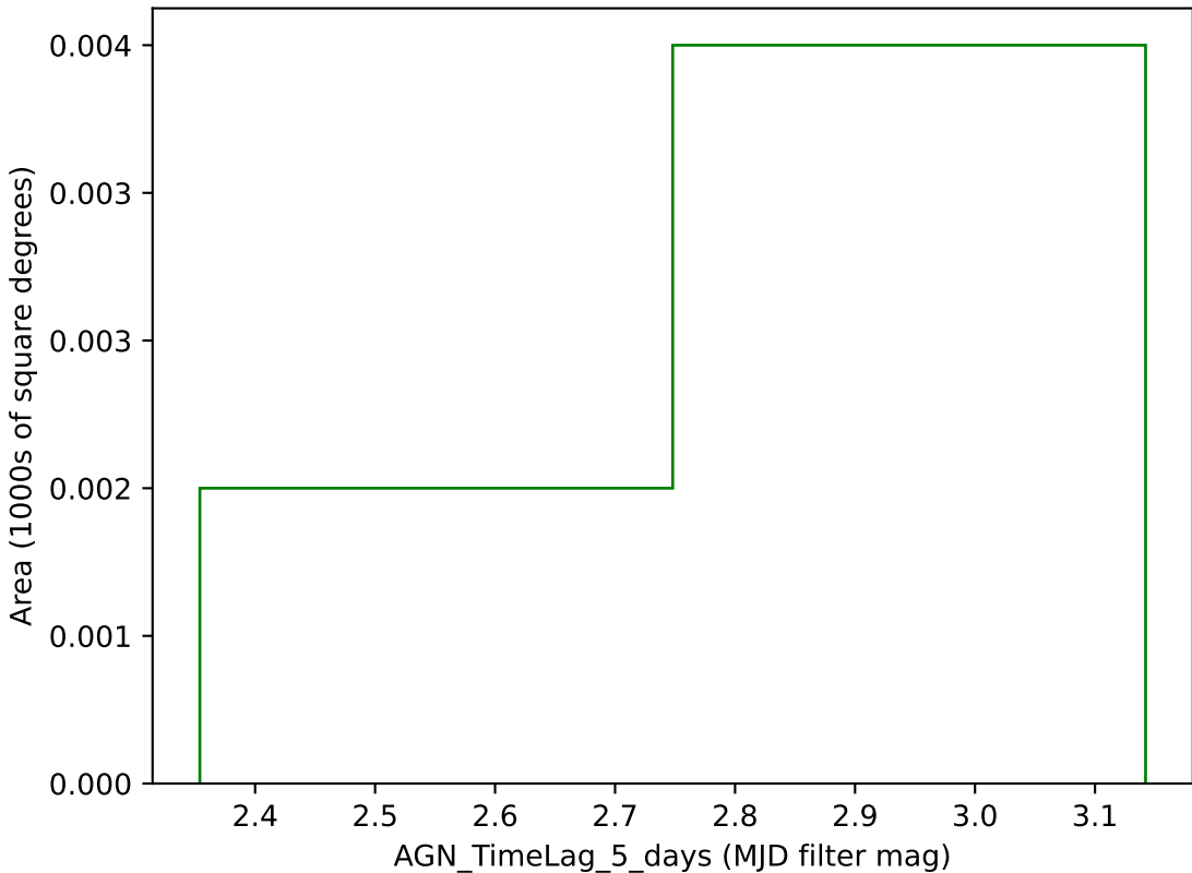
baseline_v3.4_10yrs g band: AGN_TimeLag_5_days
