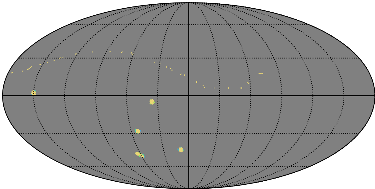
baseline_v3.4_10yrs all bands: AGN_TimeLag_5_days
