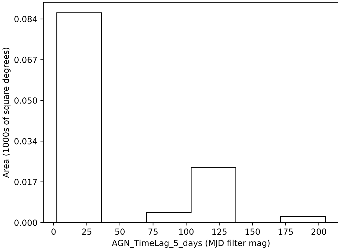
baseline_v3.4_10yrs all bands: AGN_TimeLag_5_days
