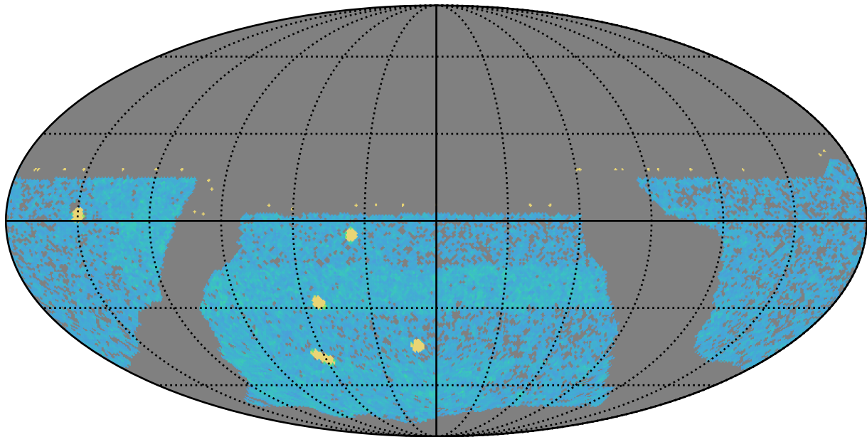
baseline_v3.4_10yrs y band: AGN_TimeLag_100_days
