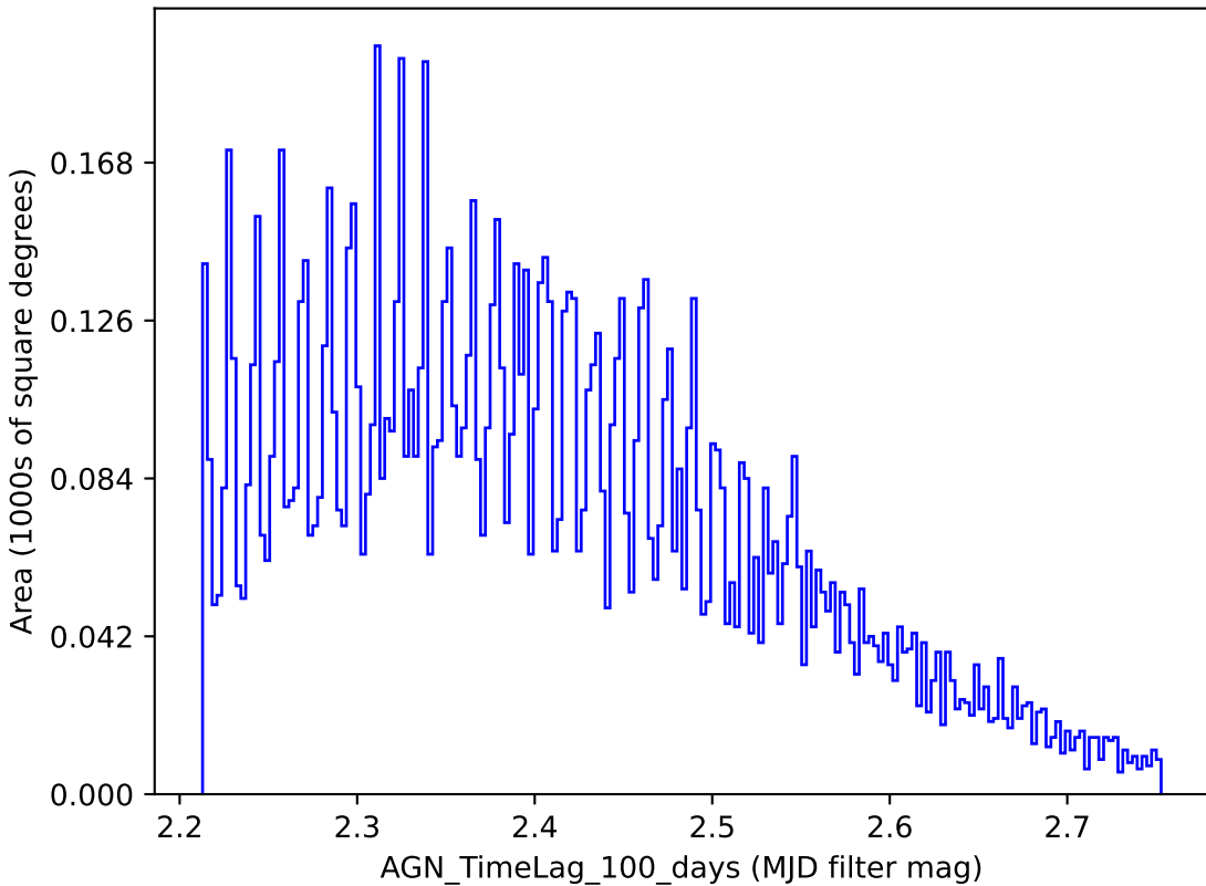
baseline_v3.4_10yrs y band: AGN_TimeLag_100_days
