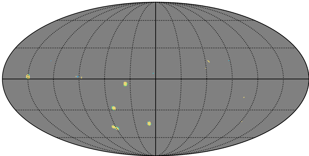
baseline_v3.4_10yrs u band: AGN_TimeLag_100_days
