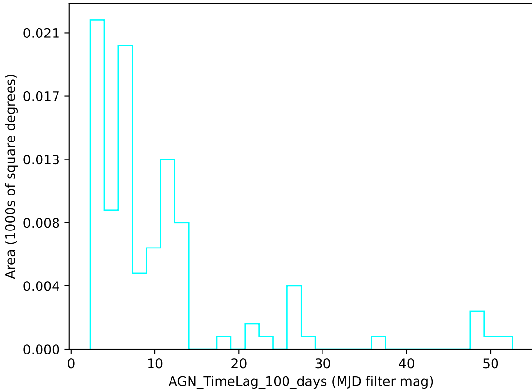
baseline_v3.4_10yrs u band: AGN_TimeLag_100_days
