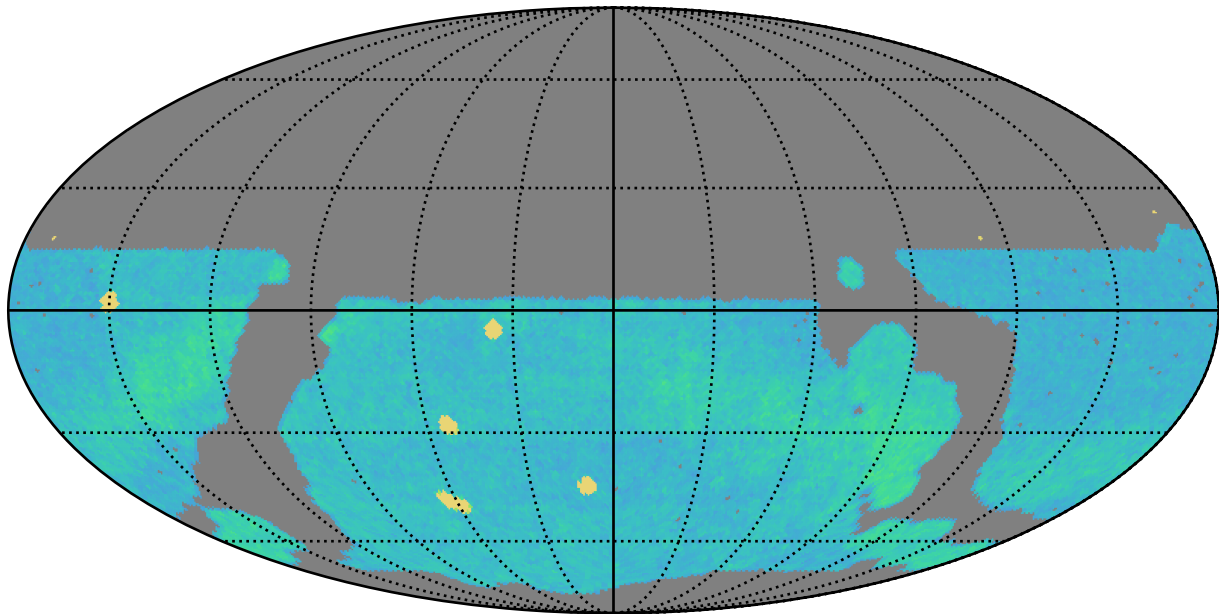
baseline_v3.4_10yrs r band: AGN_TimeLag_100_days
