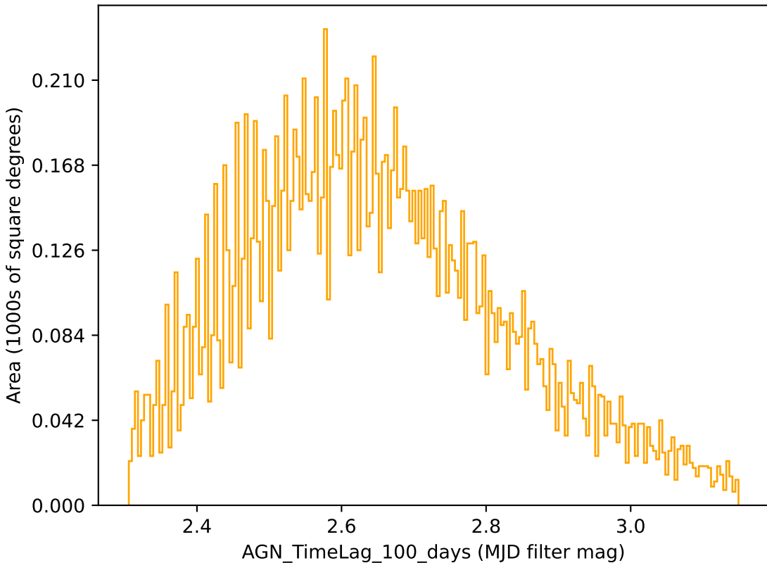
baseline_v3.4_10yrs r band: AGN_TimeLag_100_days
