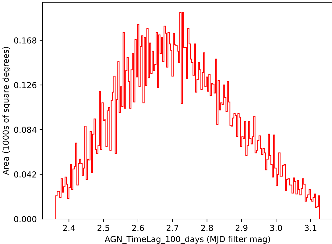
baseline_v3.4_10yrs i band: AGN_TimeLag_100_days
