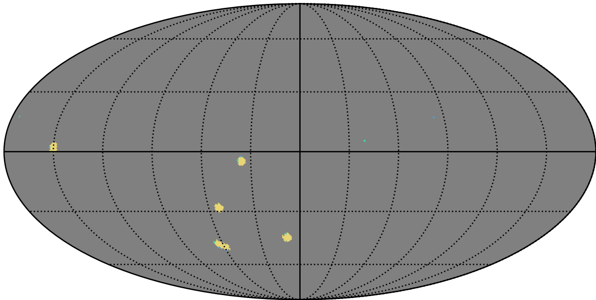
baseline_v3.4_10yrs g band: AGN_TimeLag_100_days
