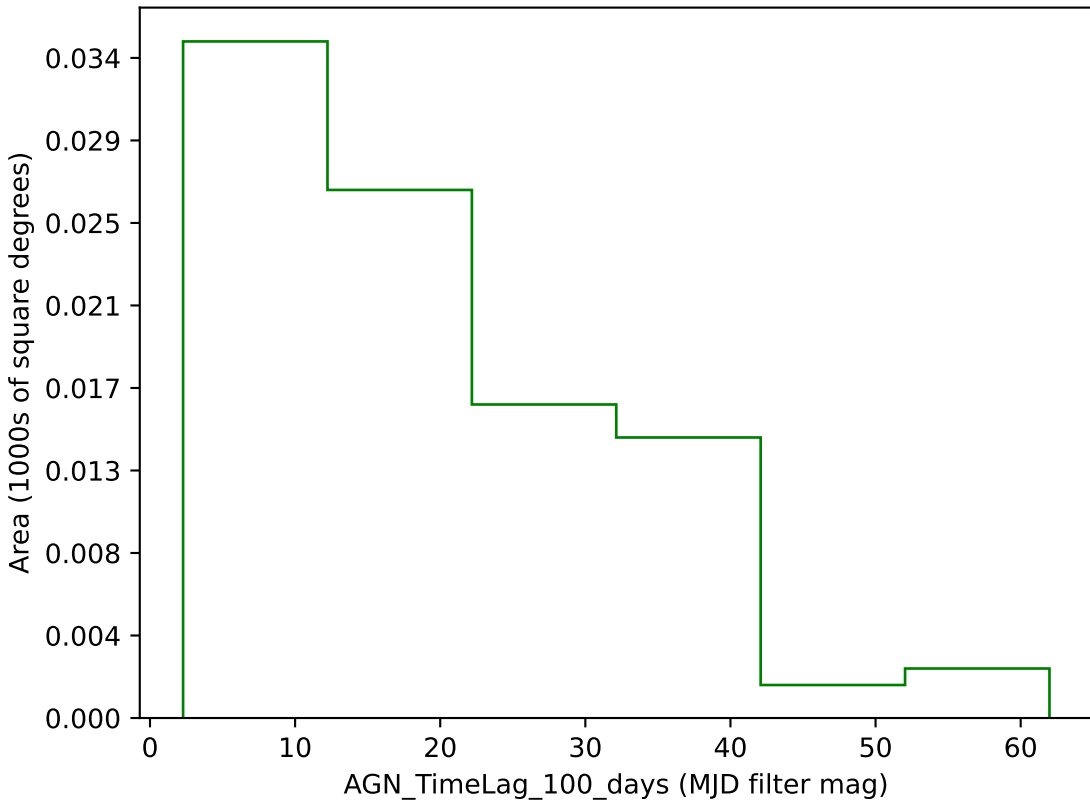
baseline_v3.4_10yrs g band: AGN_TimeLag_100_days
