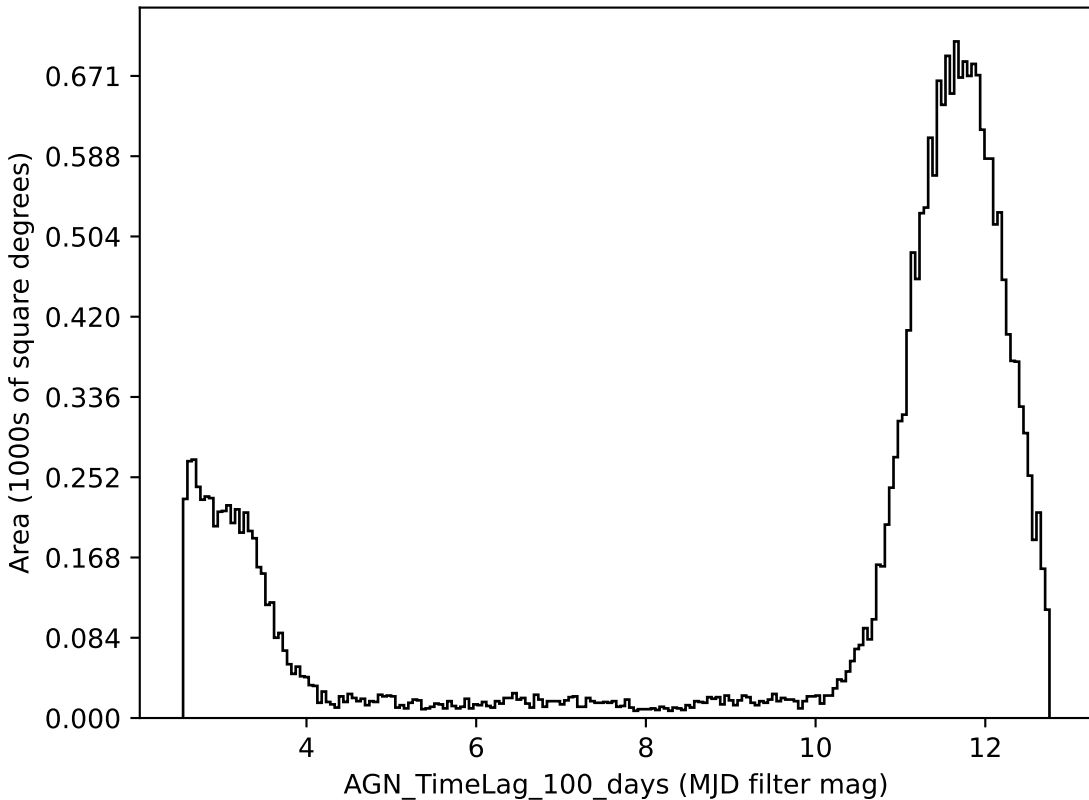
baseline_v3.4_10yrs all bands: AGN_TimeLag_100_days
