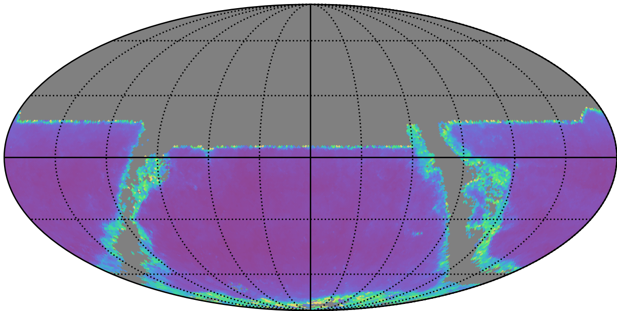
baseline_v3.4_10yrs y band: AGN SF_uncert
