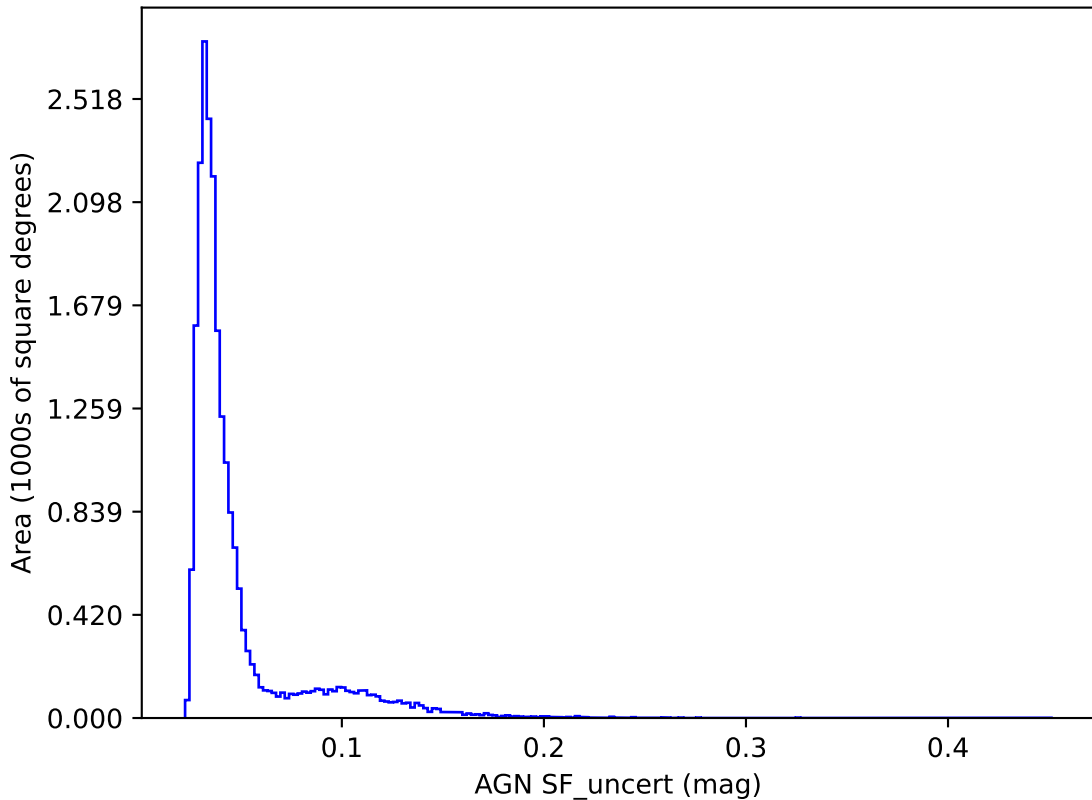
baseline_v3.4_10yrs y band: AGN SF_uncert
