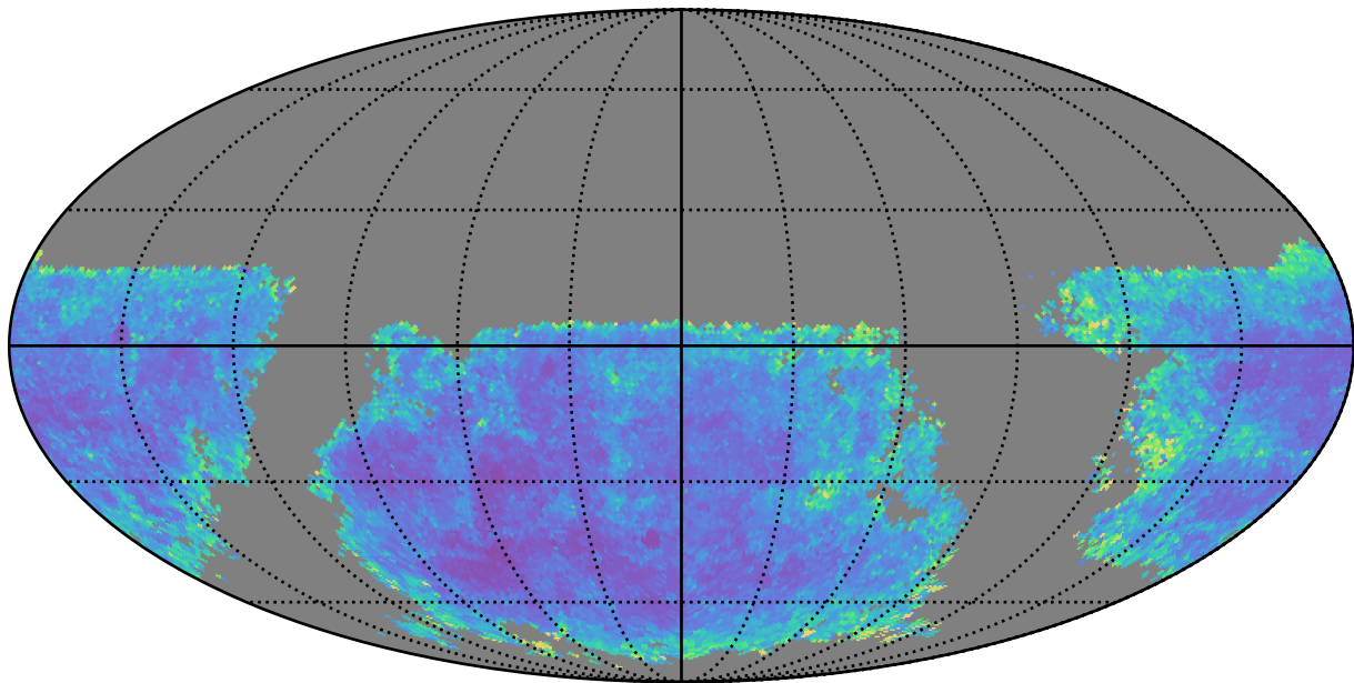
baseline_v3.4_10yrs u band: AGN SF_uncert
