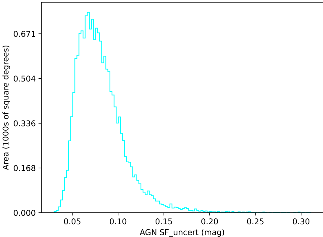
baseline_v3.4_10yrs u band: AGN SF_uncert
