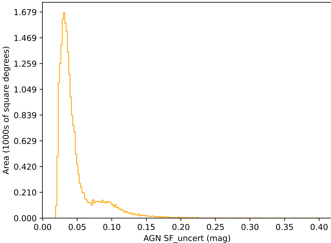
baseline_v3.4_10yrs r band: AGN SF_uncert
