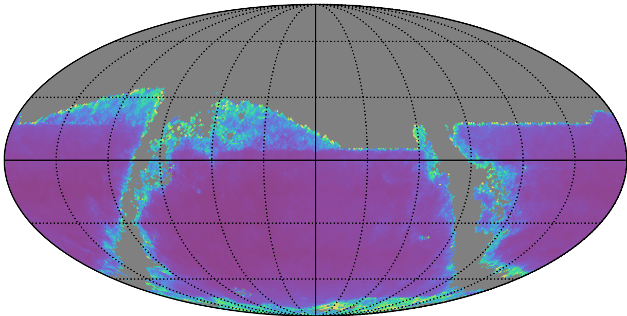
baseline_v3.4_10yrs i band: AGN SF_uncert
