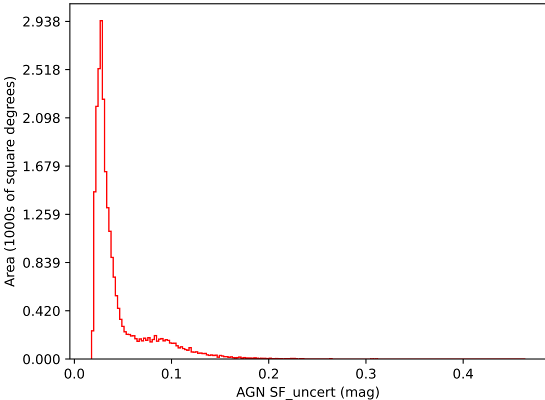
baseline_v3.4_10yrs i band: AGN SF_uncert
