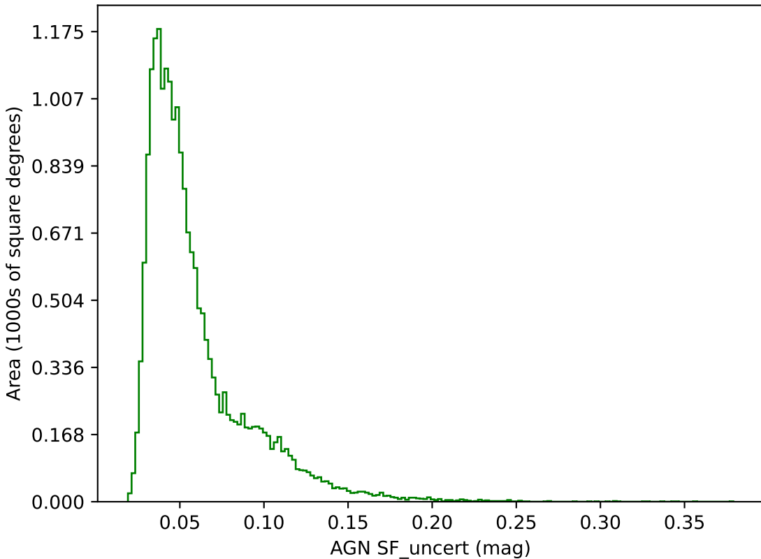
baseline_v3.4_10yrs g band: AGN SF_uncert
