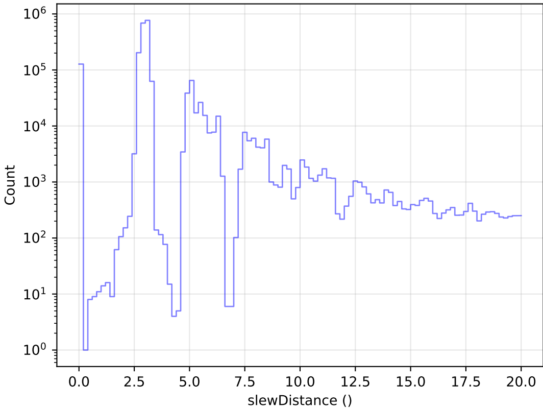
baseline_v3.4_10yrs All visits: Zoom Slew Distance Histogram
