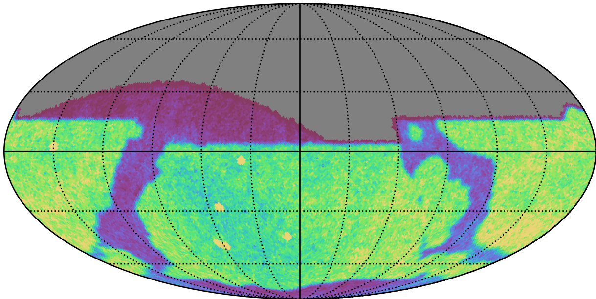
baseline_v3.4_10yrs night < 365.25: Year1.0Count
