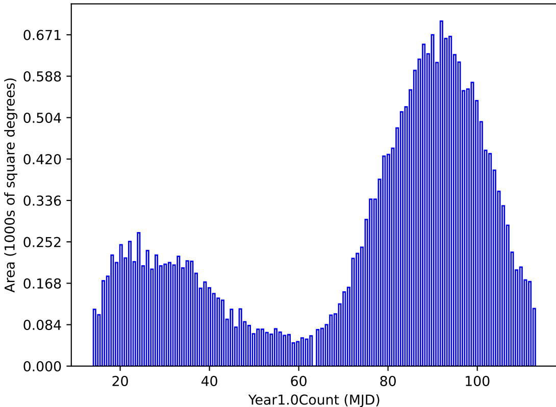
baseline_v3.4_10yrs night < 365.25: Year1.0Count
