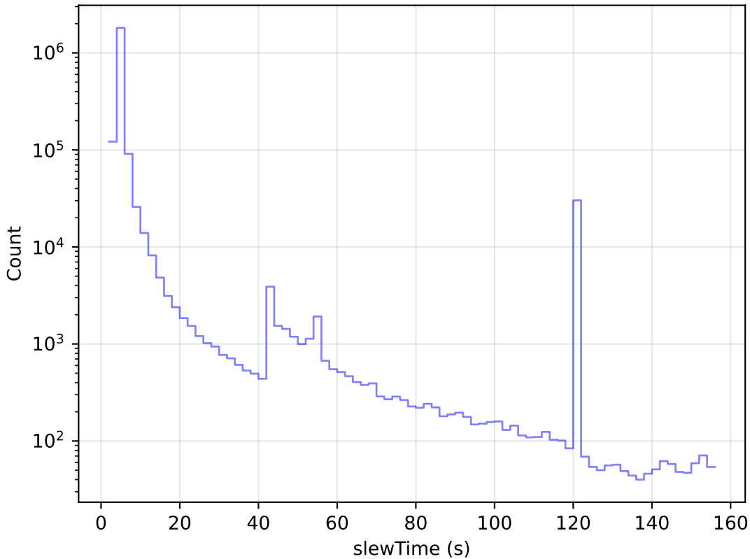
baseline_v3.4_10yrs All visits: Slew Time Histogram
