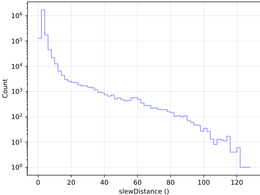
baseline_v3.4_10yrs All visits: Slew Distance Histogram
