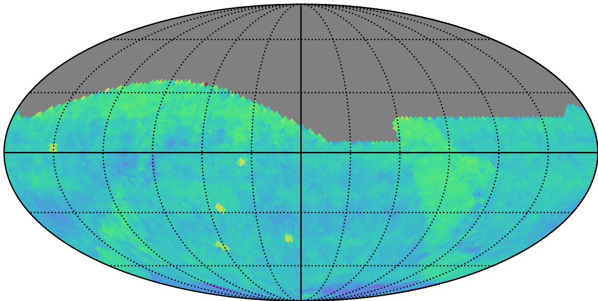
baseline_v3.4_10yrs (g or r or i): PairFraction
