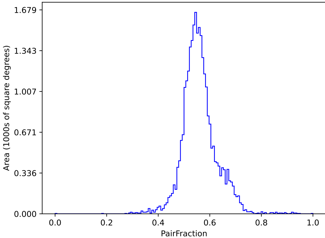
baseline_v3.4_10yrs (g or r or i): PairFraction
